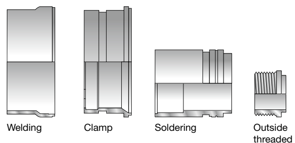
Compact flanges
