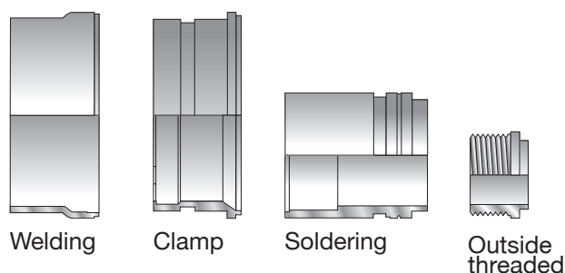
Compact flanges
